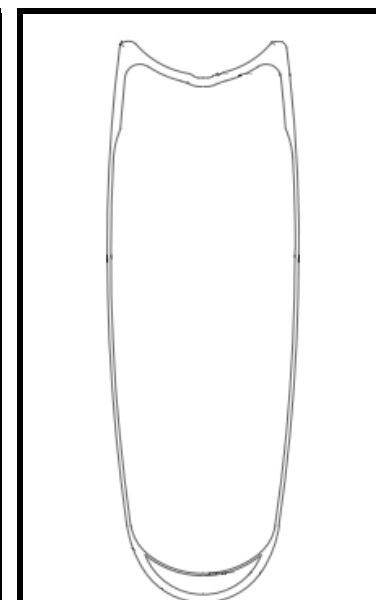
CROSS SECTION FFWD RYOT77
